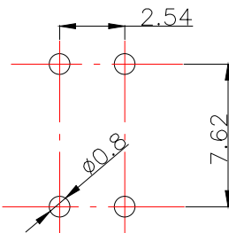
[P.C.B.LAYOUT]
