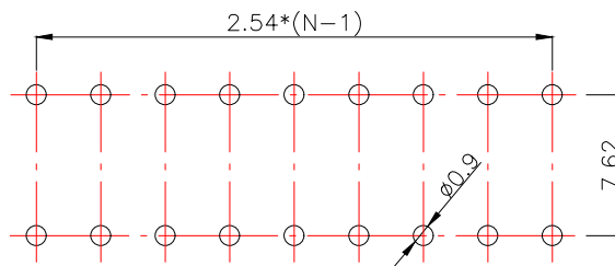
[P.C.B.LAYOUT]
