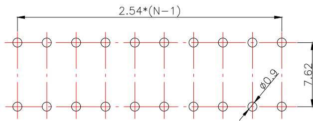
[P.C.B.LAYOUT]
