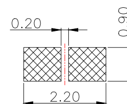
METAL MASK T=0.08
