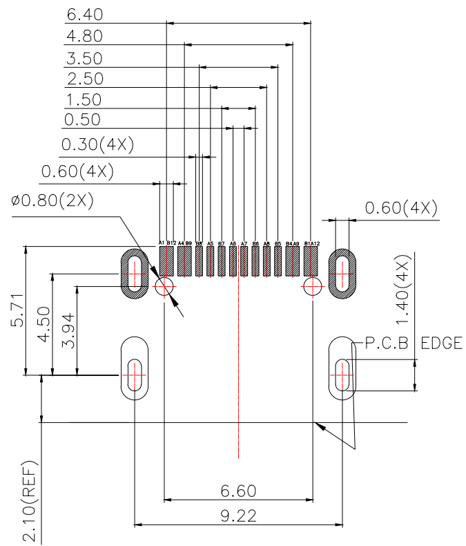
RECOMMENDED PCB LAYOUT GENERAL TOLERANCE \pm 0.05
