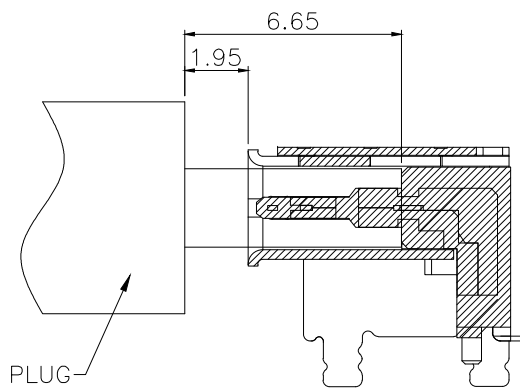
AFTER MATING SCALE 1:1
