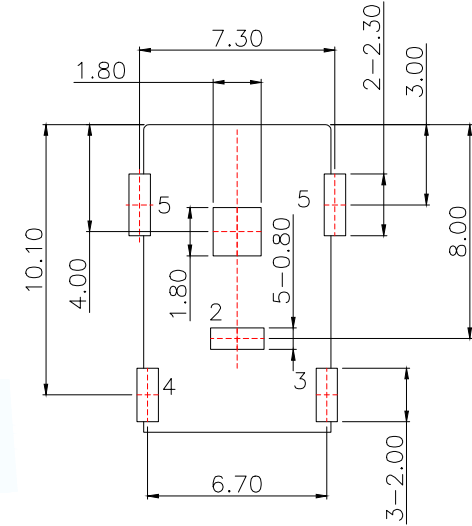
PCB.WELDING DRAWING (TOLERANCE:±0.05)
