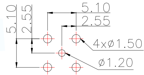
PCB.WELDING DRAWING (TOLERANCE:±0.05)
