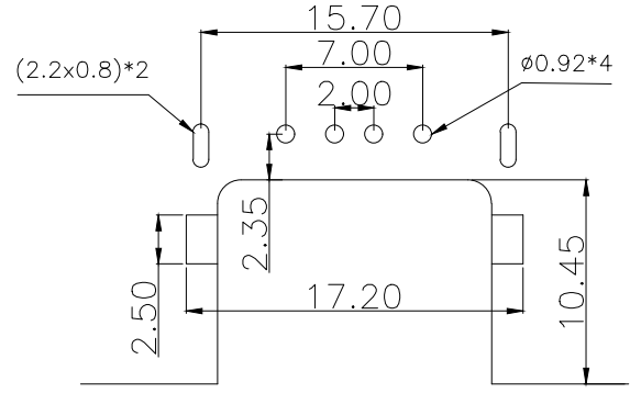
PCB.WELDING DRAWING (TOLERANCE:±0.05)
