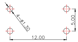
PCB.WELDING DRAWING
