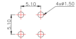
PCB.WELDING DRAWING (TOLERANCE:±0.05)
