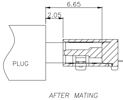
AFTER MATING
