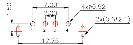
PCB.WELDING DRAWING (TOLERANCE:±0.05)
