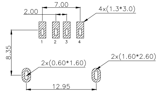
PCB.WELDING DRAWING (TOLERANCE:±0.05)
