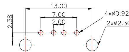
PCB.WELDING DRAWING (TOLERANCE:±0.05)
