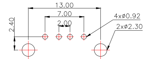
PCB.WELDING DRAWING (TOLERANCE:±0.05)
