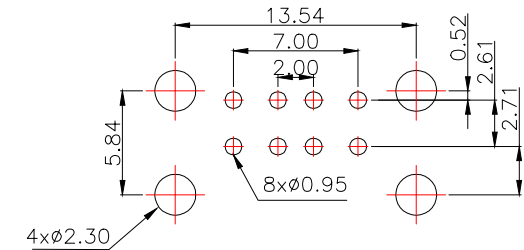
PCB.WELDING DRAWING (TOLERANCE:±0.05)
