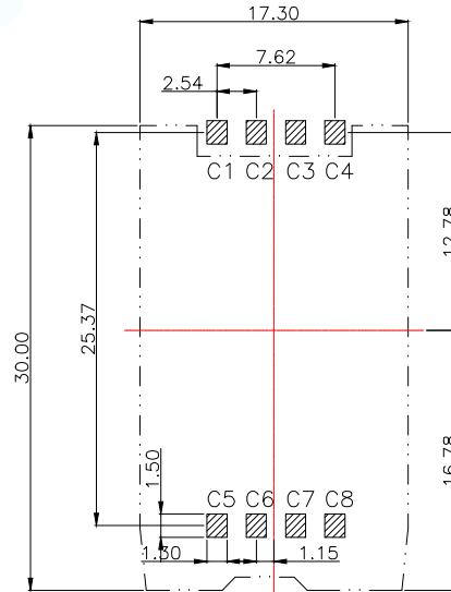
RECOMMENDED PCB LAYOUT GENERAL TOLERANCE ±0.05
