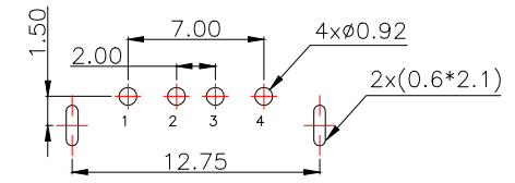
PCB.WELDING DRAWING (TOLERANCE:±0.05)
