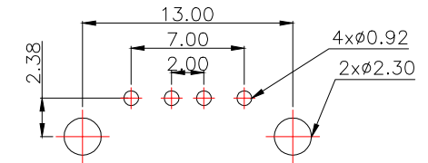
PCB.WELDING DRAWING (TOLERANCE:±0.05)
