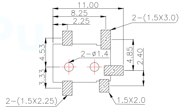
PCB.WELDING DRAWING (TOLERANCE:±0.05)
